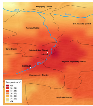
Maximum air temperature in Yakutsk, Russia (average) | 2011-2070 | RCP 4.5
